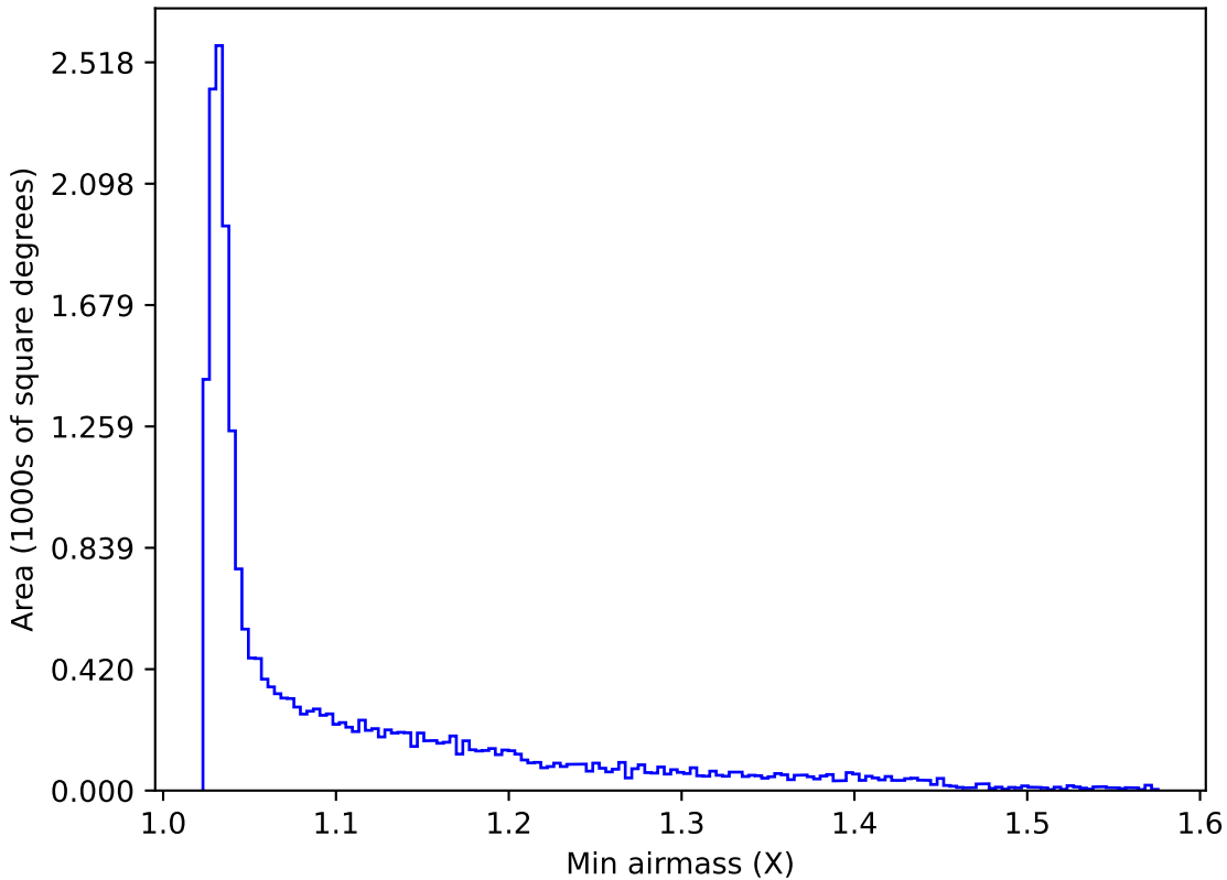
ddf_half_v3.4_10yrs All sky y band: Min airmass
