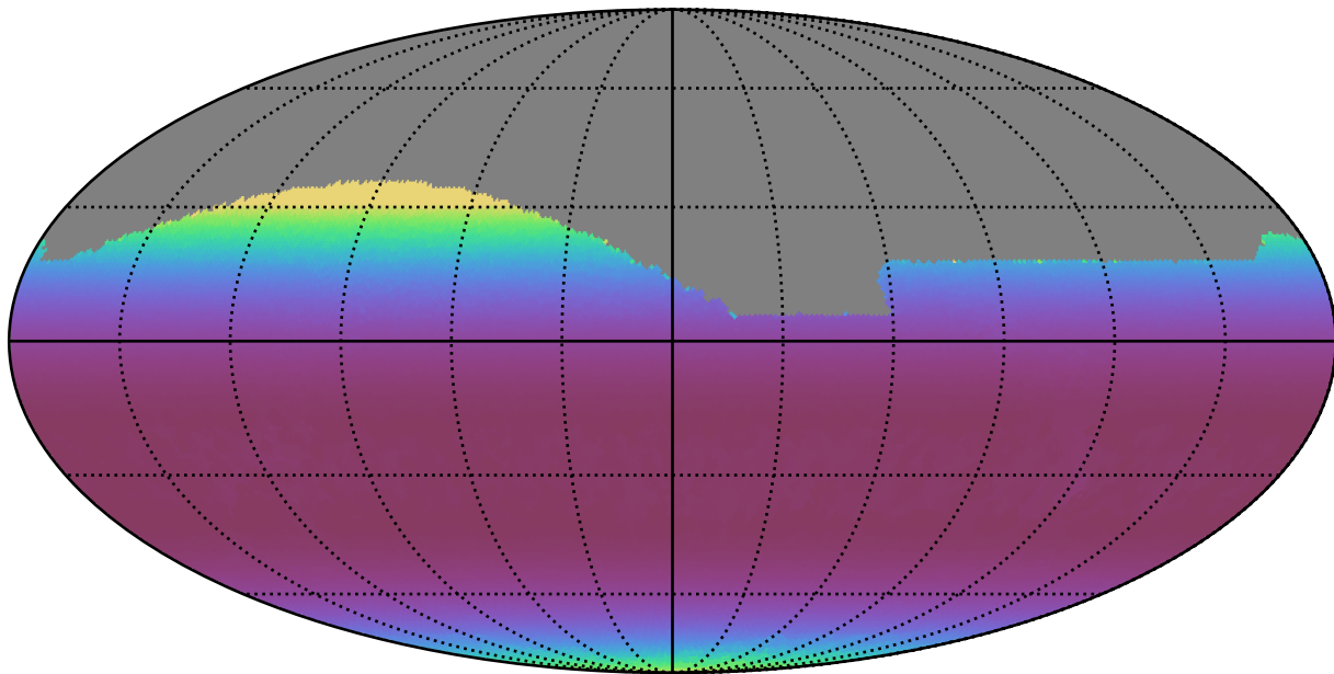
ddf_half_v3.4_10yrs All sky r band: Min airmass
