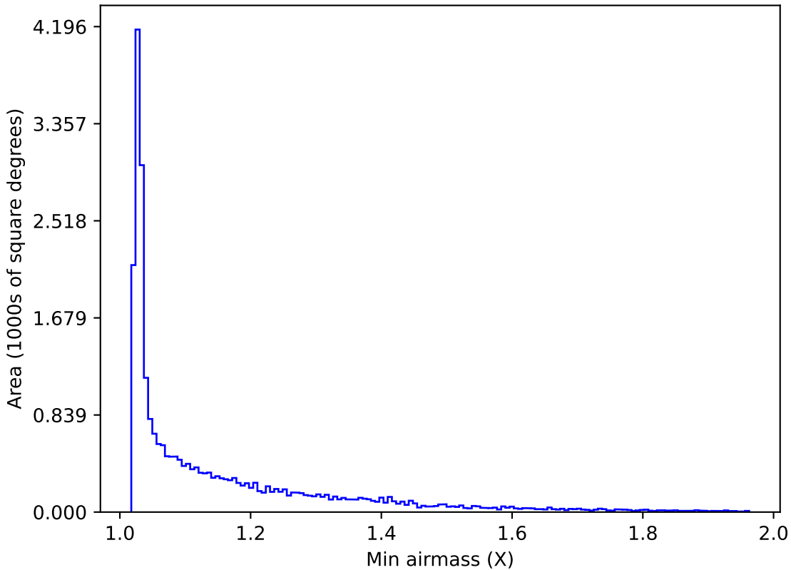
ddf_half_v3.4_10yrs All sky r band: Min airmass
