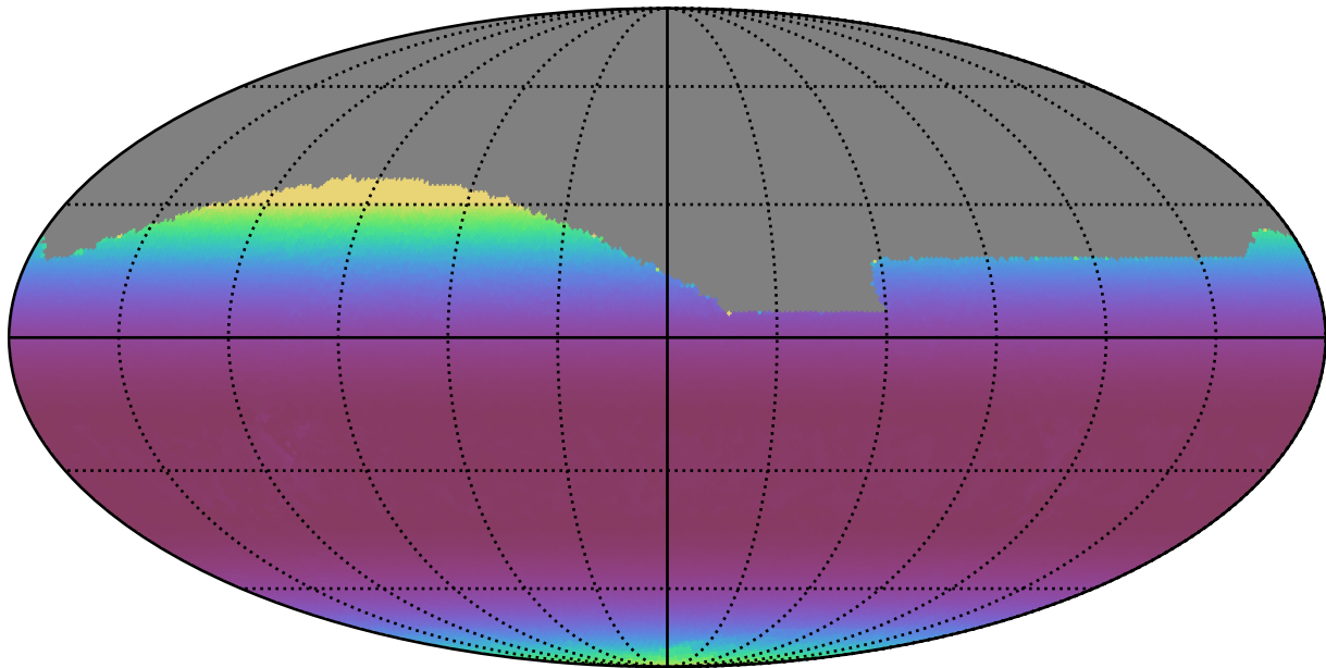
ddf_half_v3.4_10yrs All sky i band: Min airmass
