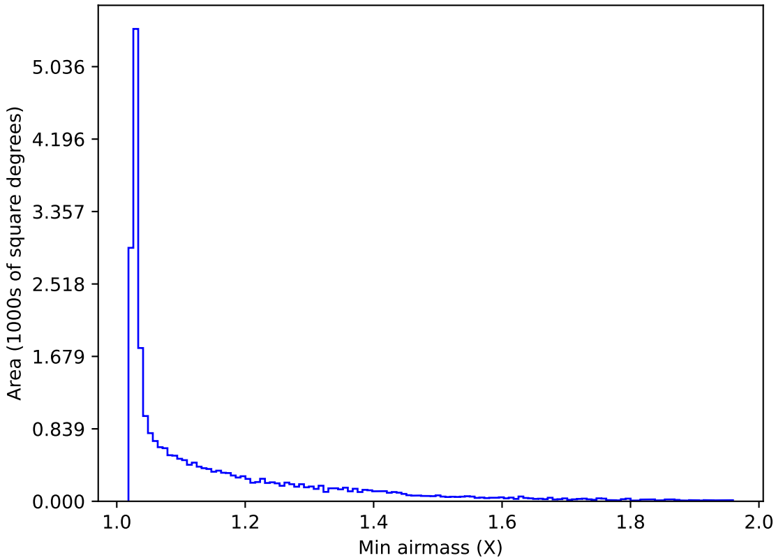
ddf_half_v3.4_10yrs All sky i band: Min airmass
