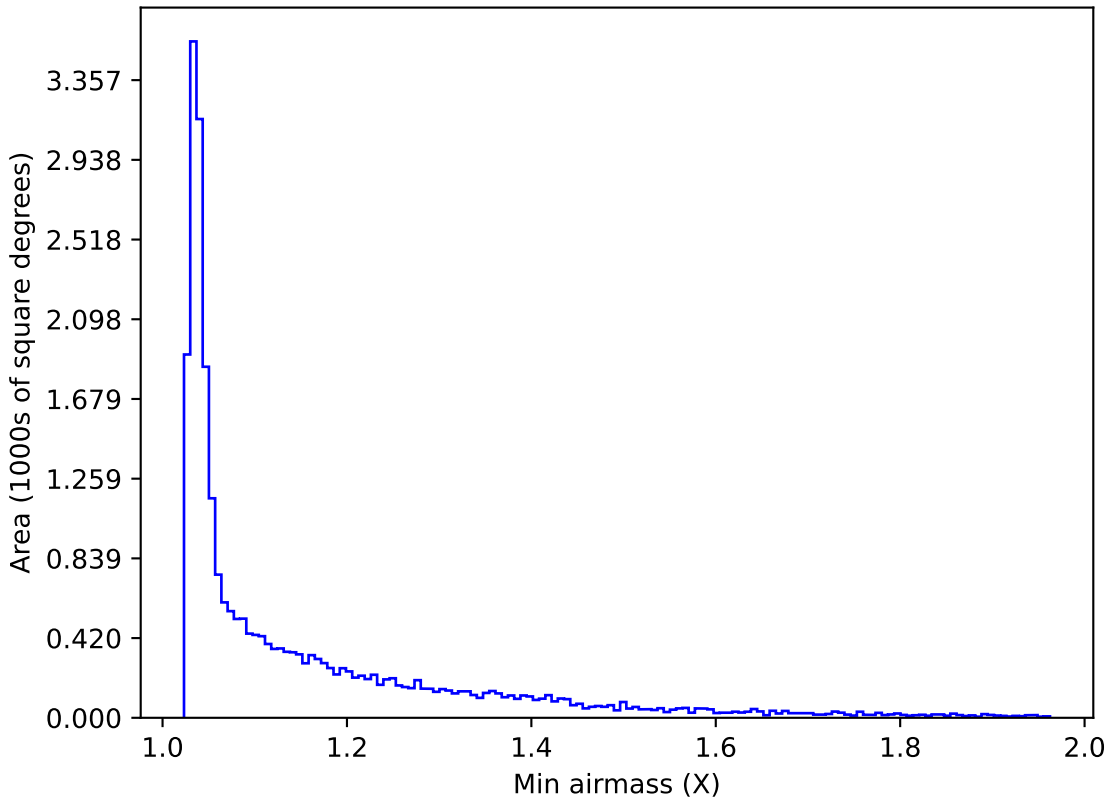
ddf_half_v3.4_10yrs All sky g band: Min airmass
