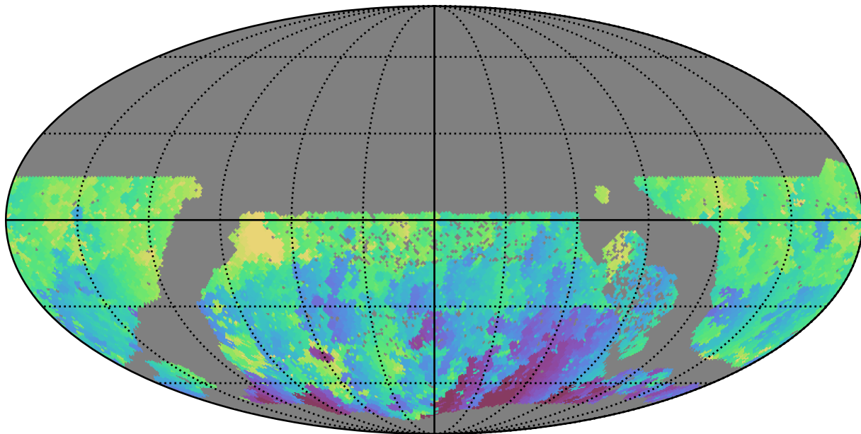
ddf_half_v3.4_10yrs WFD u band: Min HA
