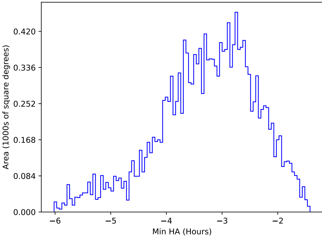
ddf_half_v3.4_10yrs WFD u band: Min HA
