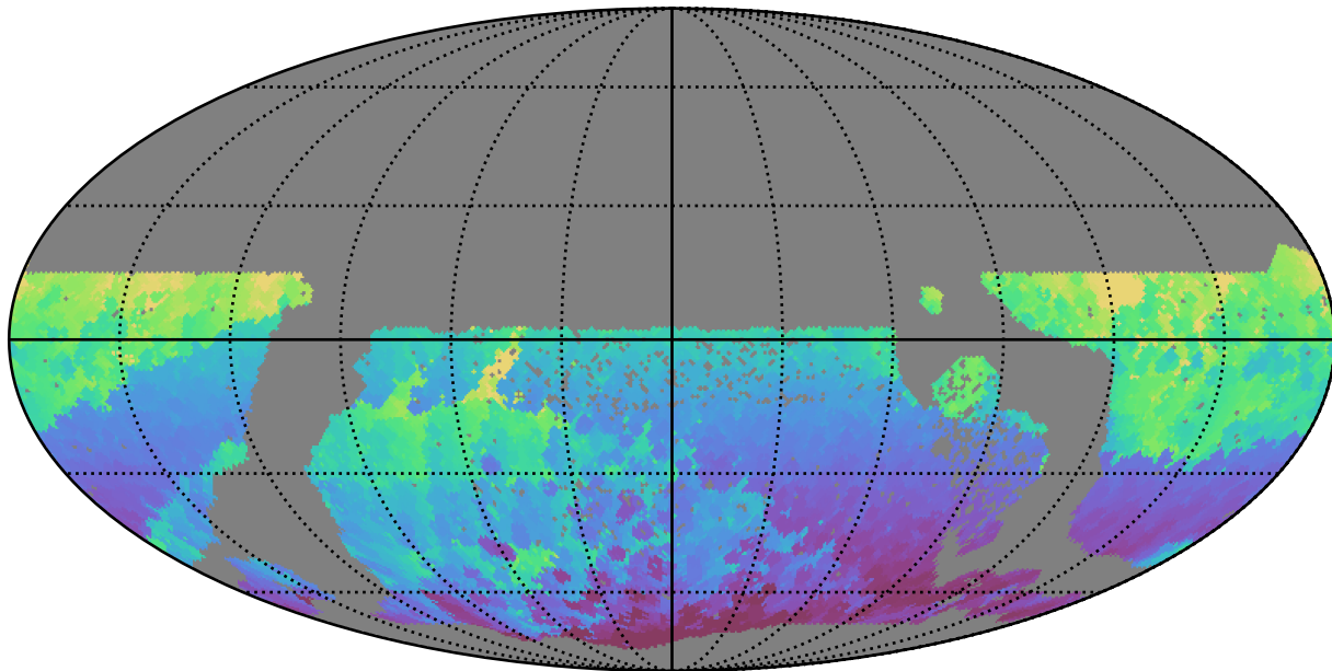
ddf_half_v3.4_10yrs WFD r band: Min HA
