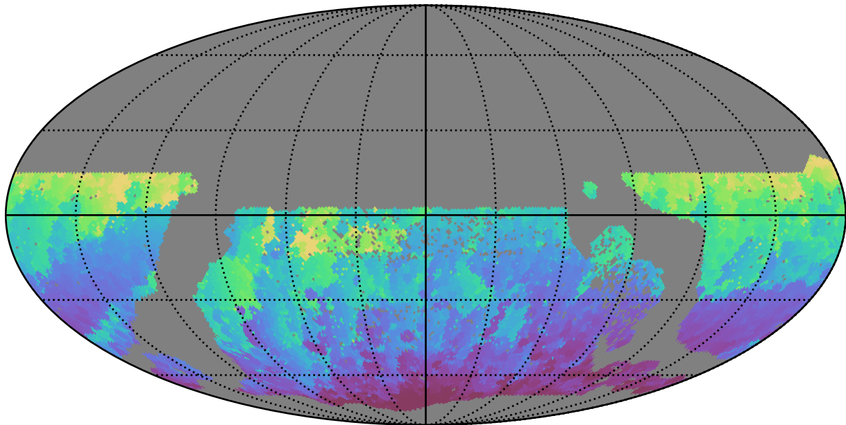
ddf_half_v3.4_10yrs WFD i band: Min HA
