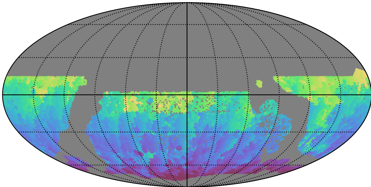
ddf_half_v3.4_10yrs WFD g band: Min HA
