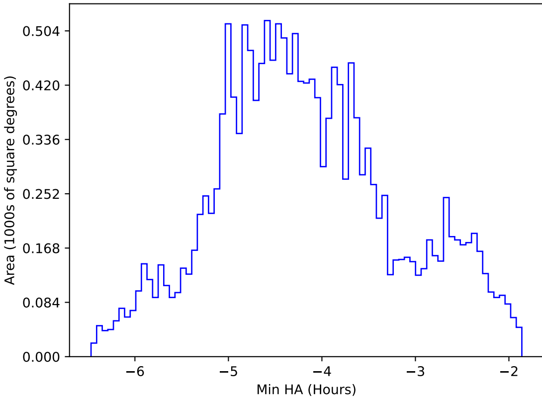
ddf_half_v3.4_10yrs WFD g band: Min HA
