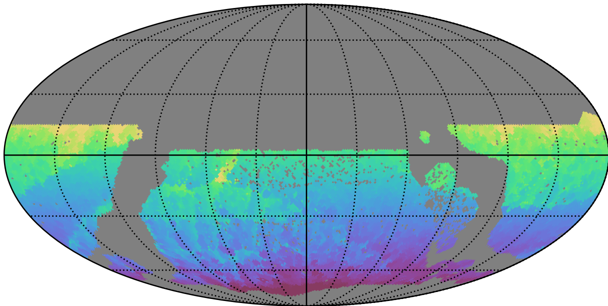
ddf_half_v3.4_10yrs WFD all bands: Min HA
