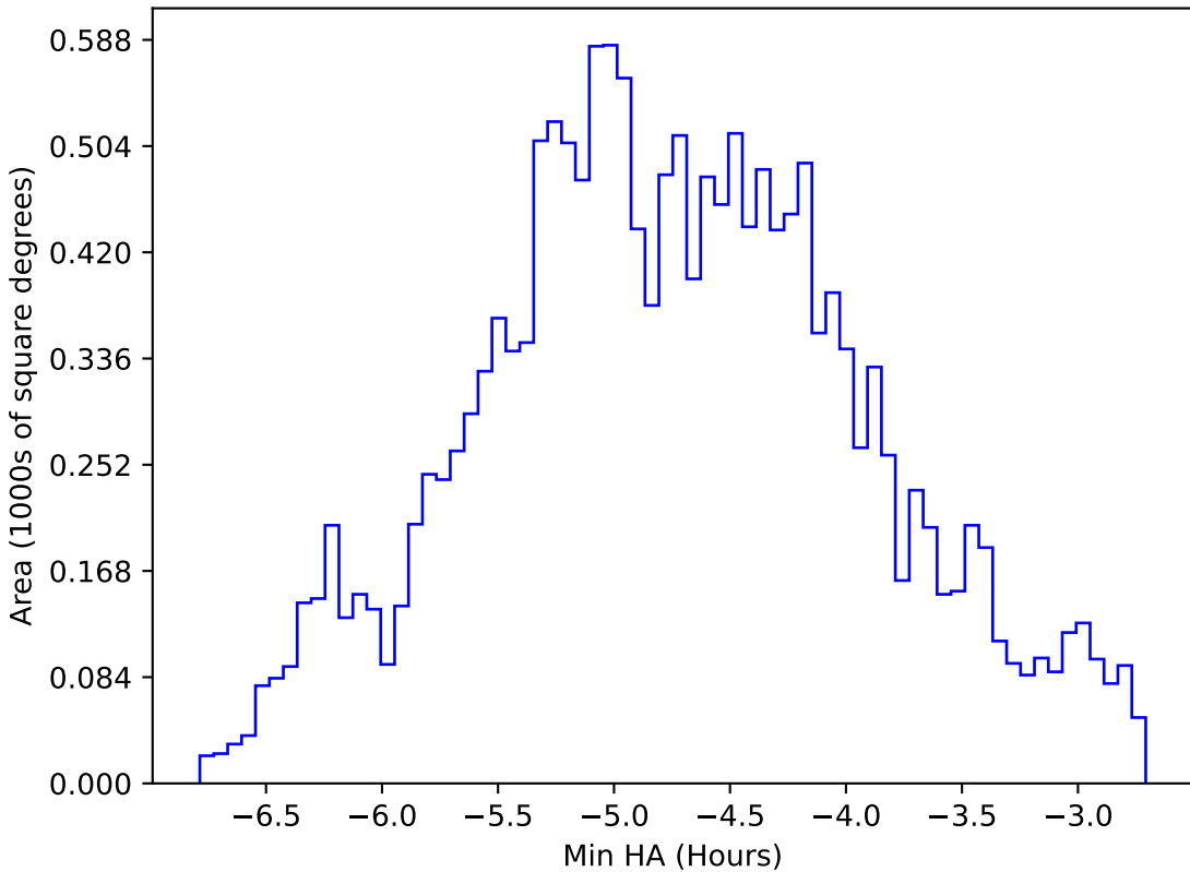
ddf_half_v3.4_10yrs WFD all bands: Min HA
