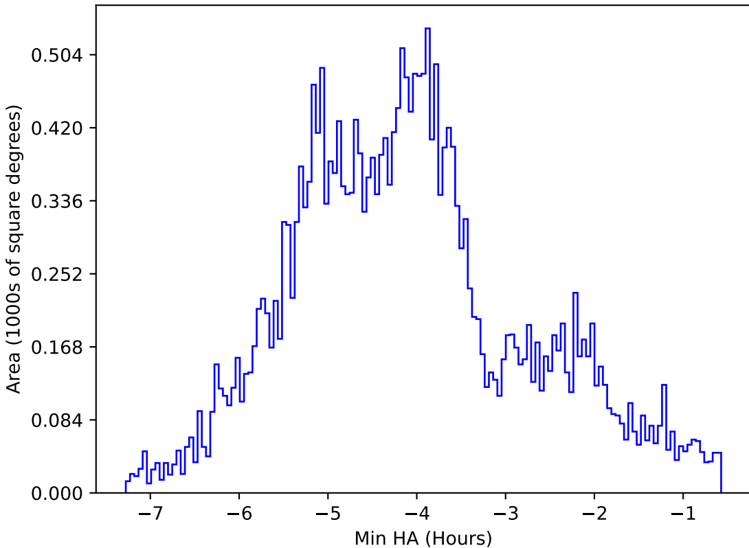
ddf_half_v3.4_10yrs All sky z band: Min HA
