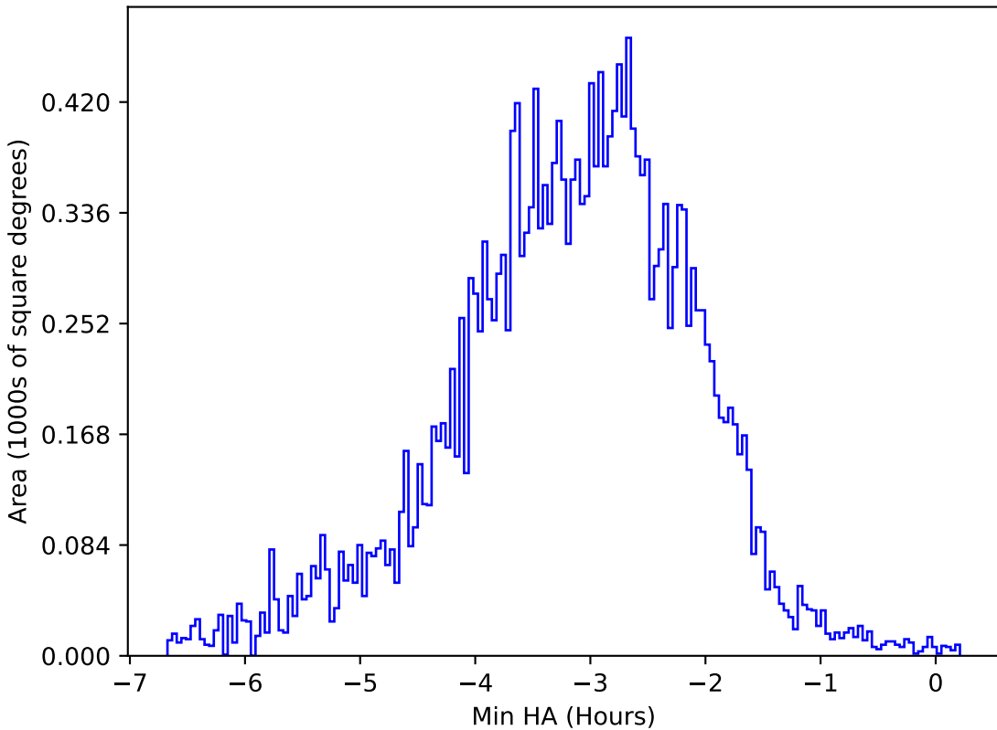
ddf_half_v3.4_10yrs All sky u band: Min HA
