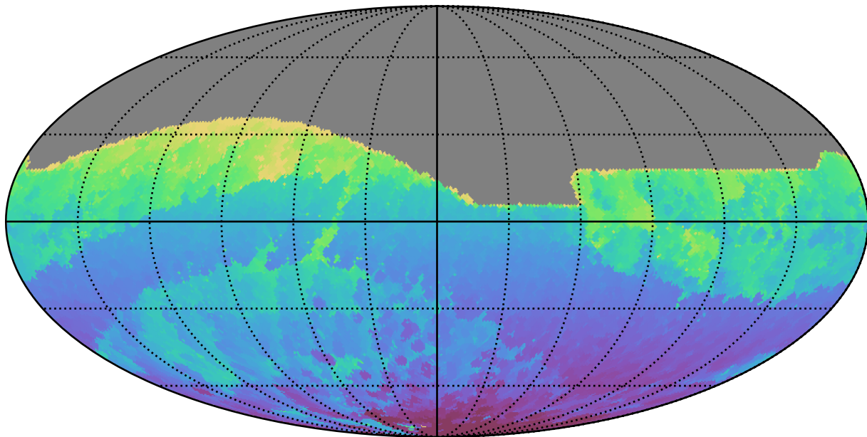
ddf_half_v3.4_10yrs All sky r band: Min HA
