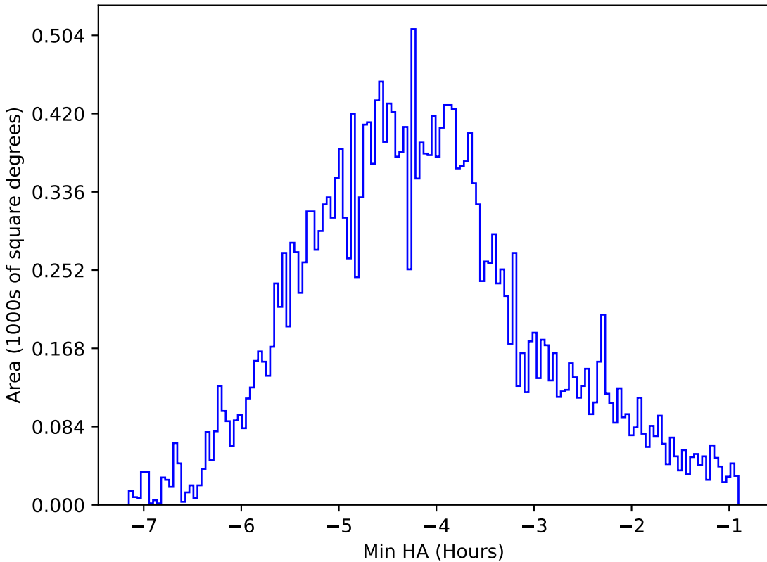
ddf_half_v3.4_10yrs All sky r band: Min HA
