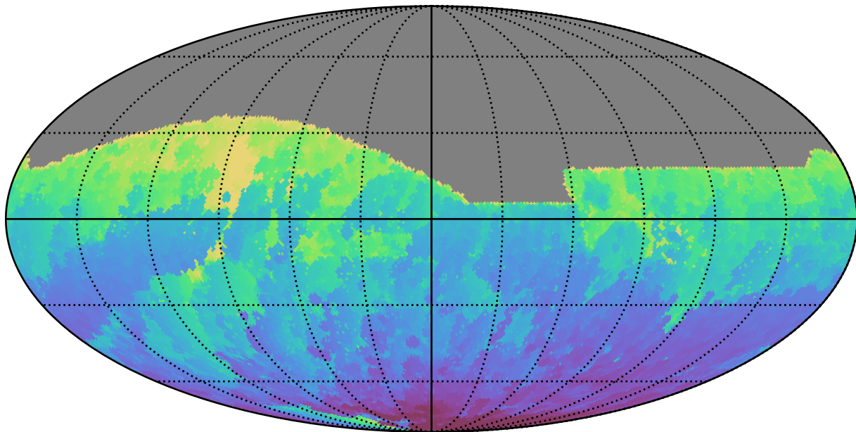
ddf_half_v3.4_10yrs All sky i band: Min HA
