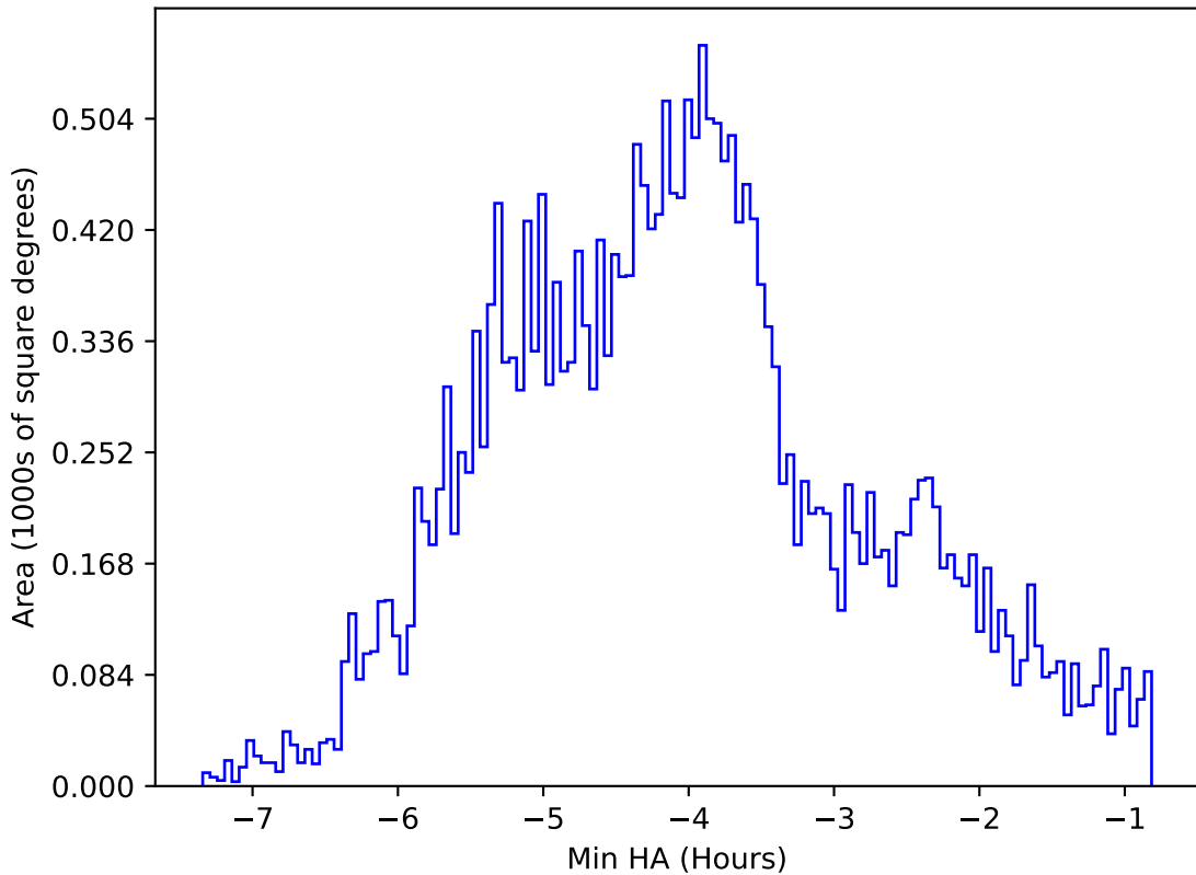
ddf_half_v3.4_10yrs All sky i band: Min HA
