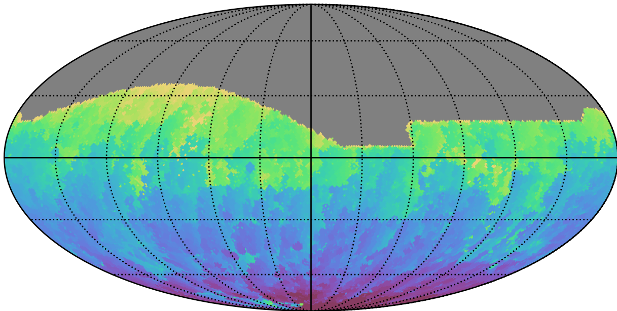
ddf_half_v3.4_10yrs All sky g band: Min HA
