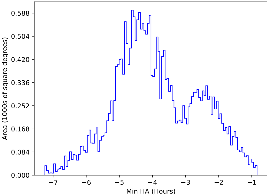
ddf_half_v3.4_10yrs All sky g band: Min HA
