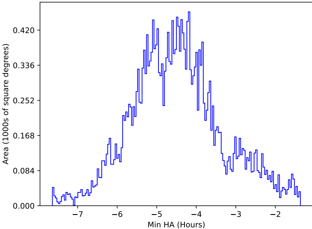
ddf_half_v3.4_10yrs All sky all bands: Min HA
