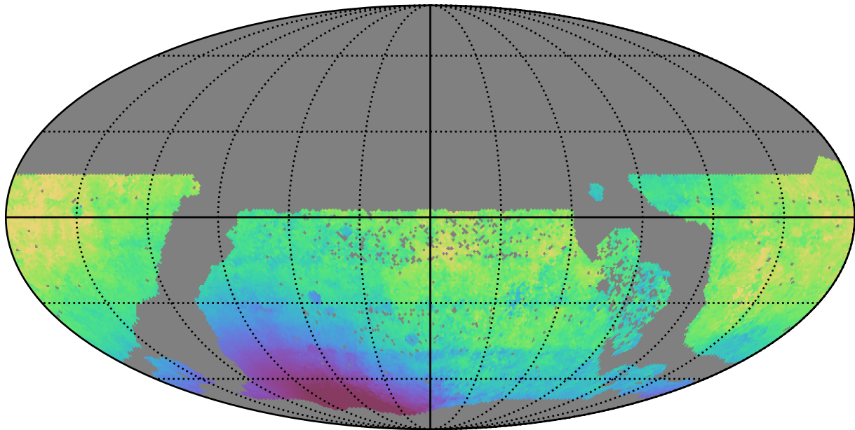
ddf_half_v3.4_10yrs WFD z band: Median solarElong
