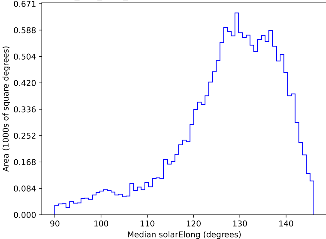
ddf_half_v3.4_10yrs WFD z band: Median solarElong
