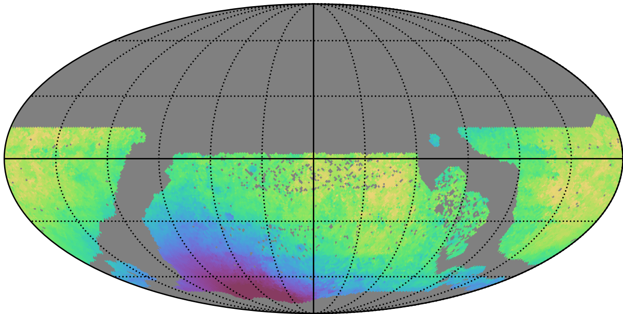
ddf_half_v3.4_10yrs WFD y band: Median solarElong
