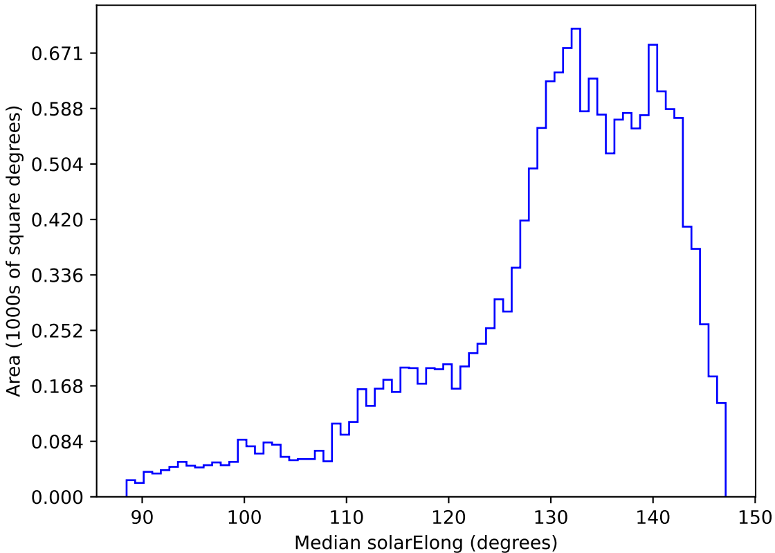
ddf_half_v3.4_10yrs WFD y band: Median solarElong
