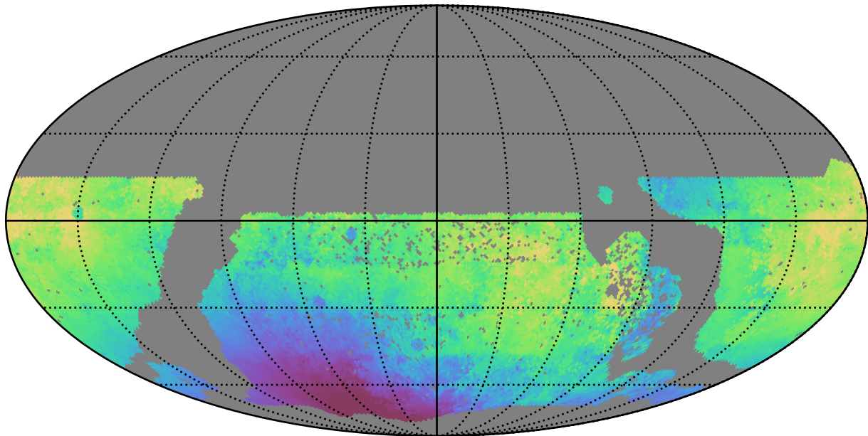
ddf_half_v3.4_10yrs WFD u band: Median solarElong
