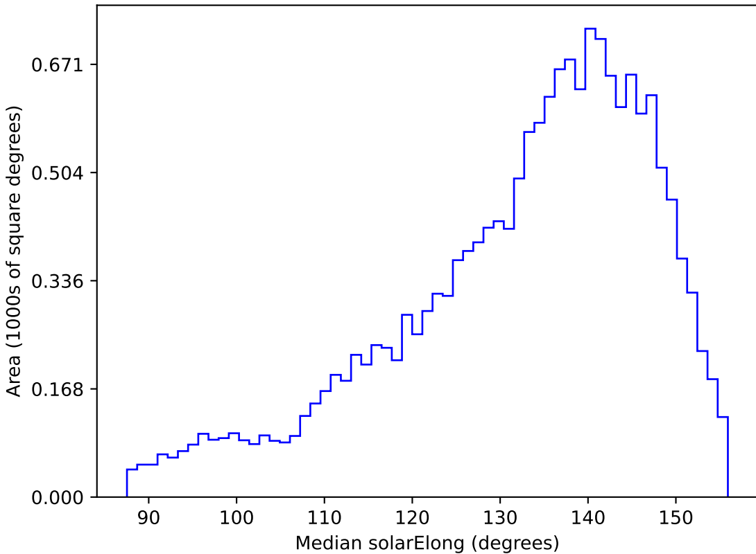
ddf_half_v3.4_10yrs WFD u band: Median solarElong
