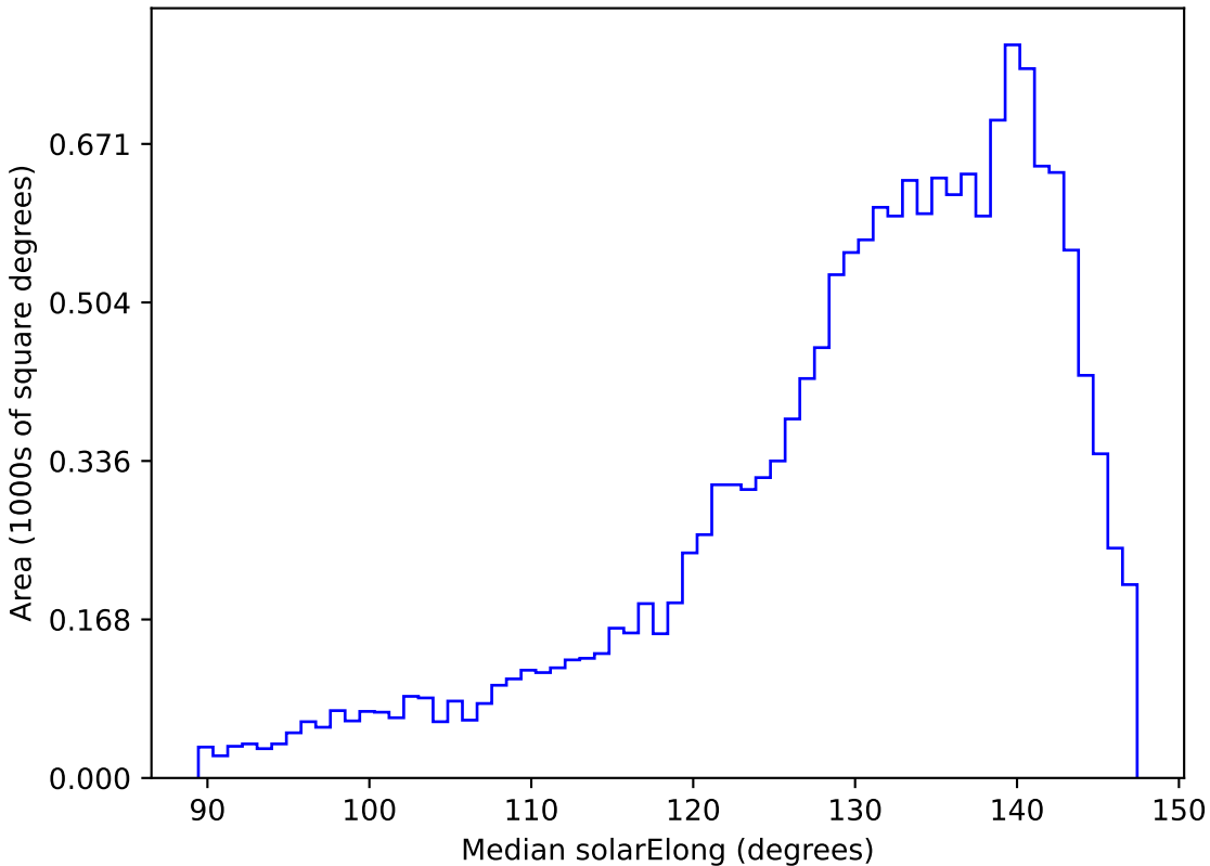
ddf_half_v3.4_10yrs WFD r band: Median solarElong
