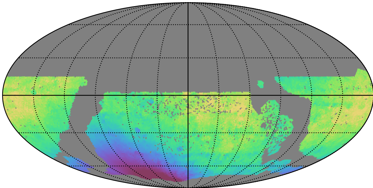
ddf_half_v3.4_10yrs WFD i band: Median solarElong
