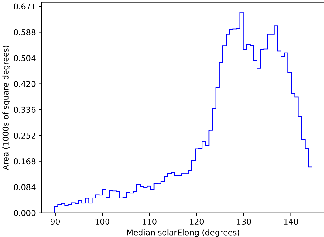
ddf_half_v3.4_10yrs WFD i band: Median solarElong
