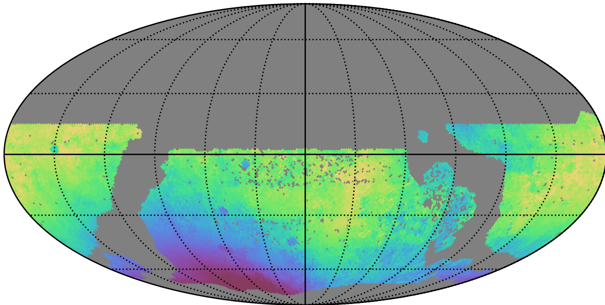
ddf_half_v3.4_10yrs WFD g band: Median solarElong
