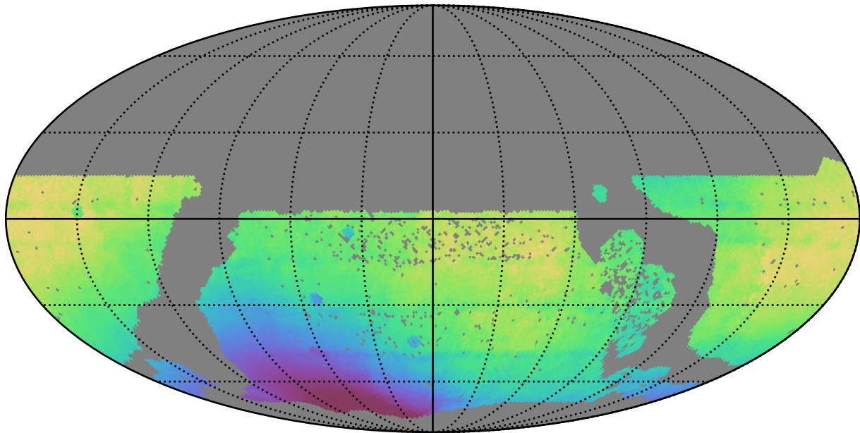
ddf_half_v3.4_10yrs WFD all bands: Median solarElong
