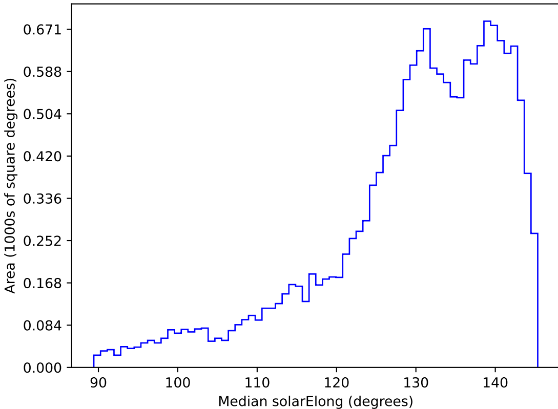
ddf_half_v3.4_10yrs WFD all bands: Median solarElong
