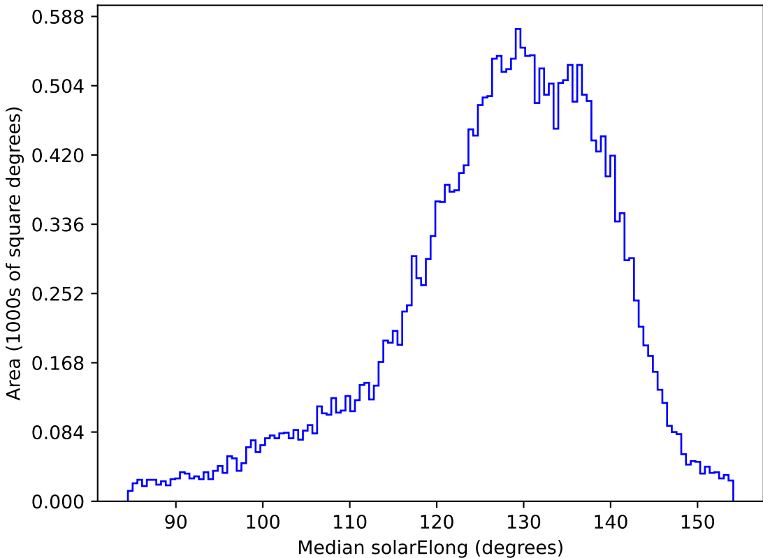
ddf_half_v3.4_10yrs All sky z band: Median solarElong
