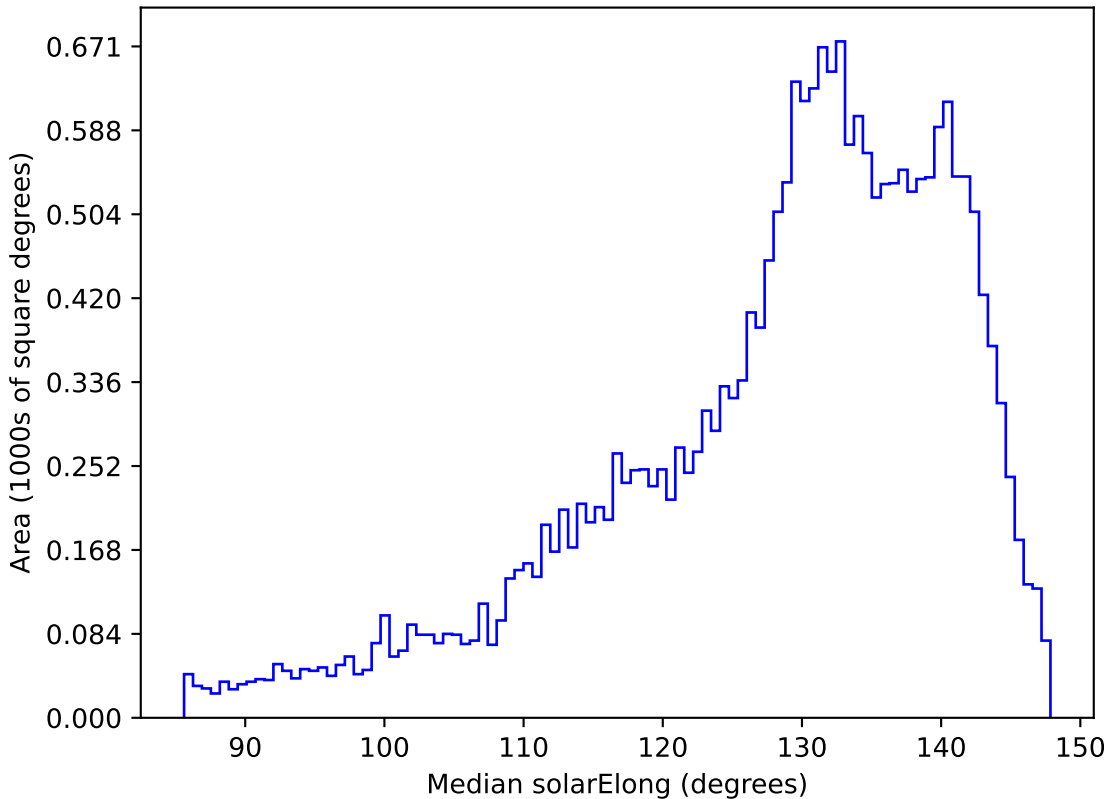
ddf_half_v3.4_10yrs All sky y band: Median solarElong
