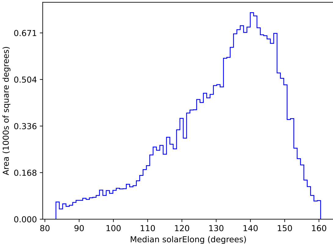
ddf_half_v3.4_10yrs All sky u band: Median solarElong
