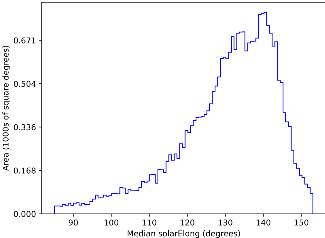
ddf_half_v3.4_10yrs All sky r band: Median solarElong
