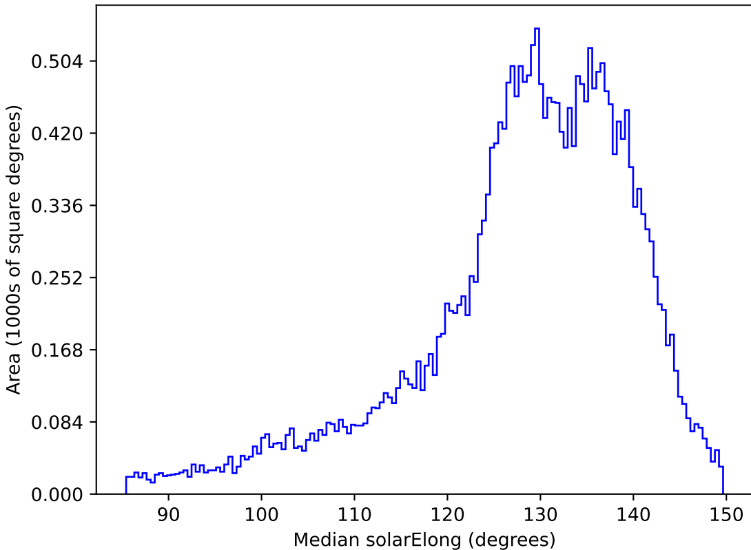
ddf_half_v3.4_10yrs All sky i band: Median solarElong
