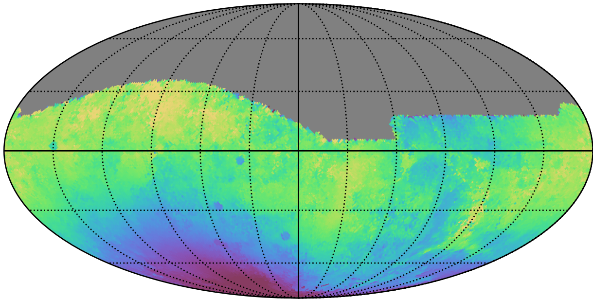
ddf_half_v3.4_10yrs All sky g band: Median solarElong
