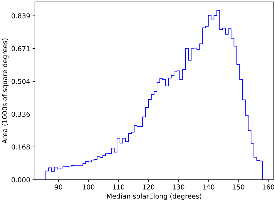
ddf_half_v3.4_10yrs All sky g band: Median solarElong
