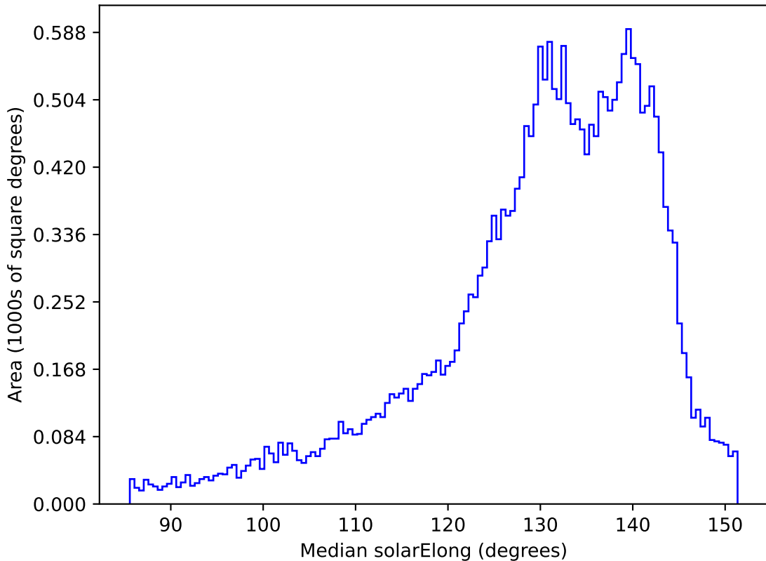
ddf_half_v3.4_10yrs All sky all bands: Median solarElong
