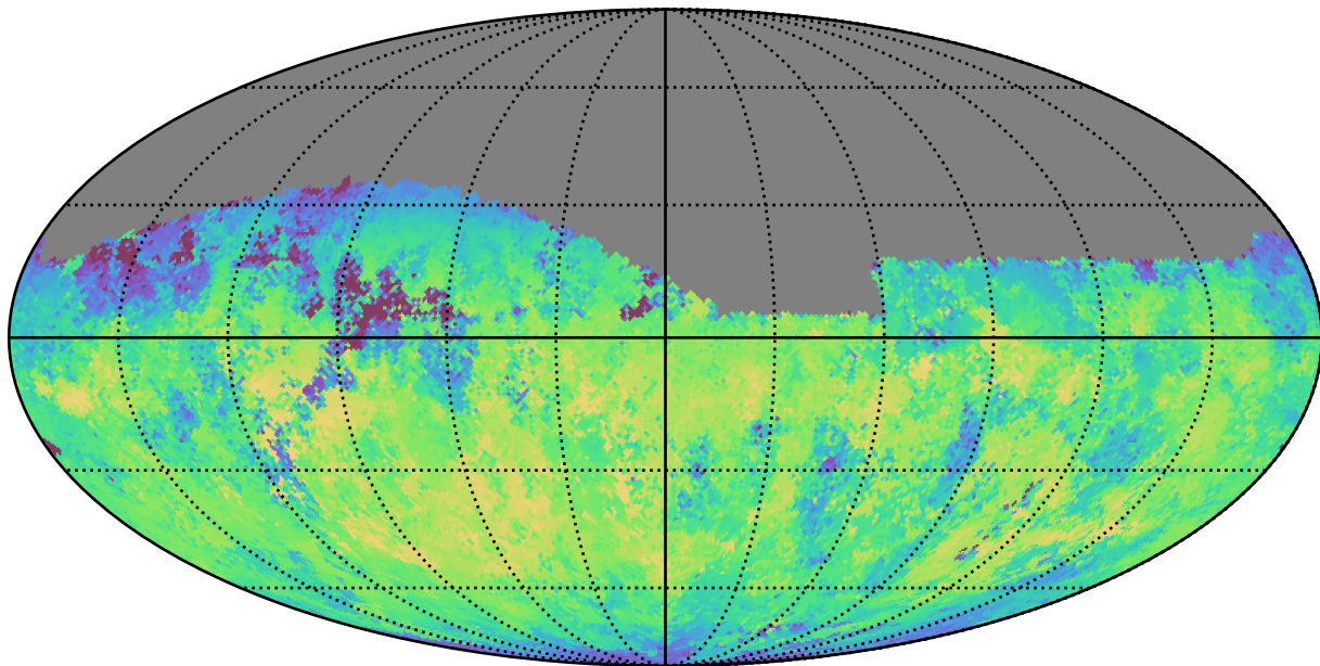
ddf_half_v3.4_10yrs Yr 1 z band: Median skyBrightness
