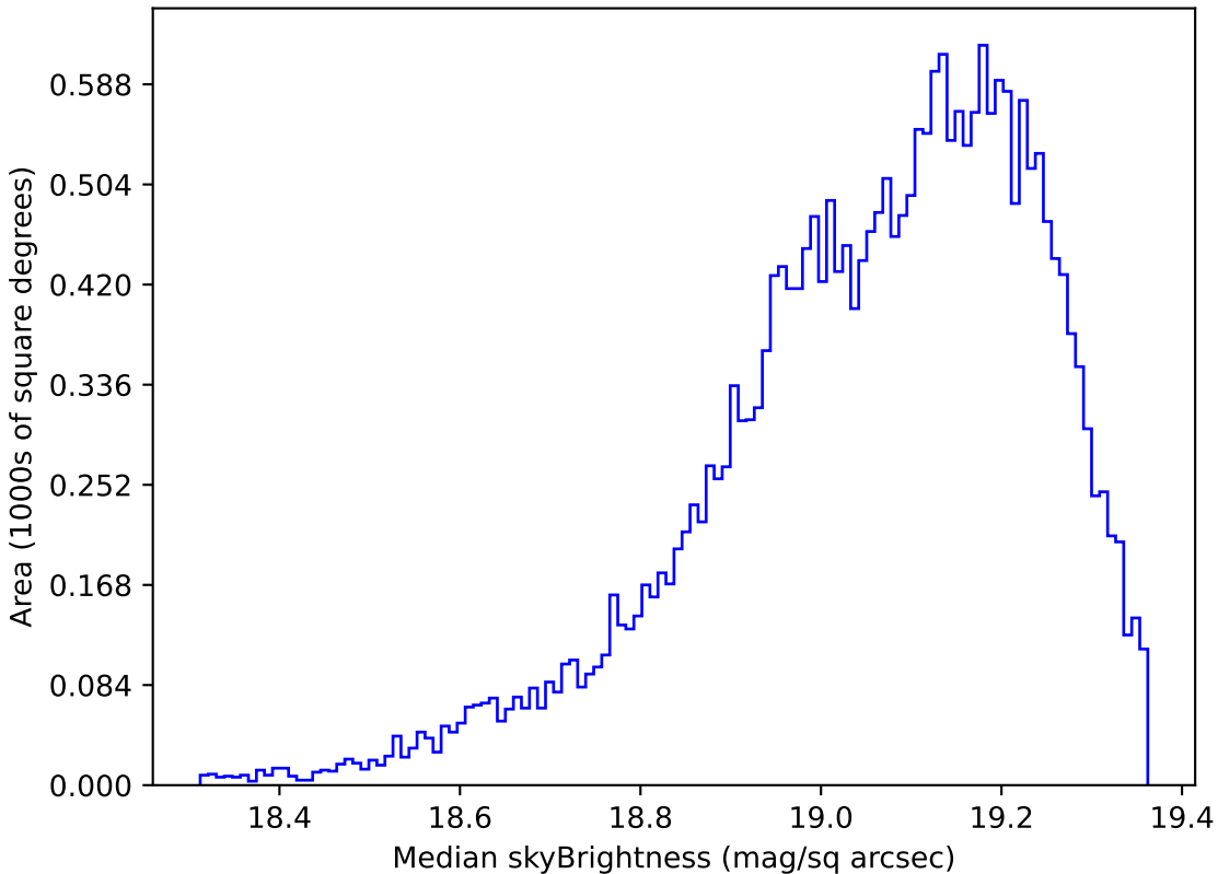
ddf_half_v3.4_10yrs Yr 1 z band: Median skyBrightness
