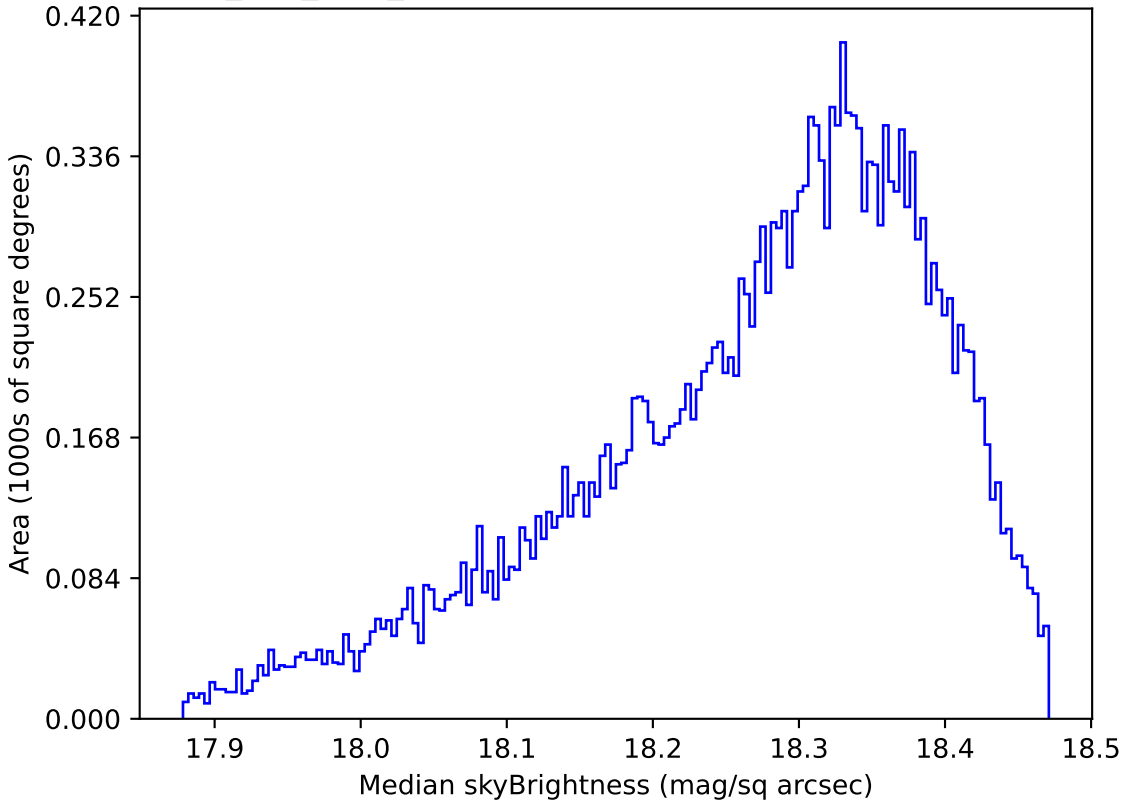
ddf_half_v3.4_10yrs Yr 1 y band: Median skyBrightness
