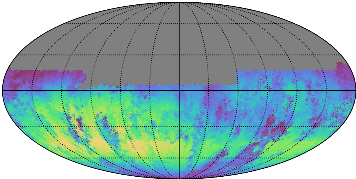
ddf_half_v3.4_10yrs Yr 1 u band: Median skyBrightness
