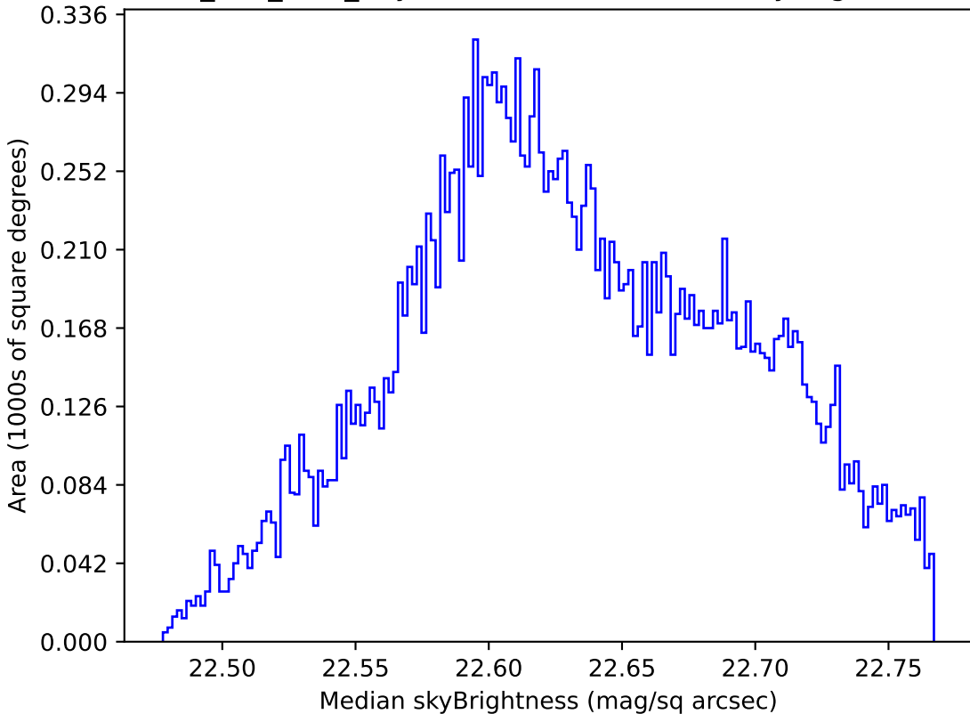
ddf_half_v3.4_10yrs Yr 1 u band: Median skyBrightness
