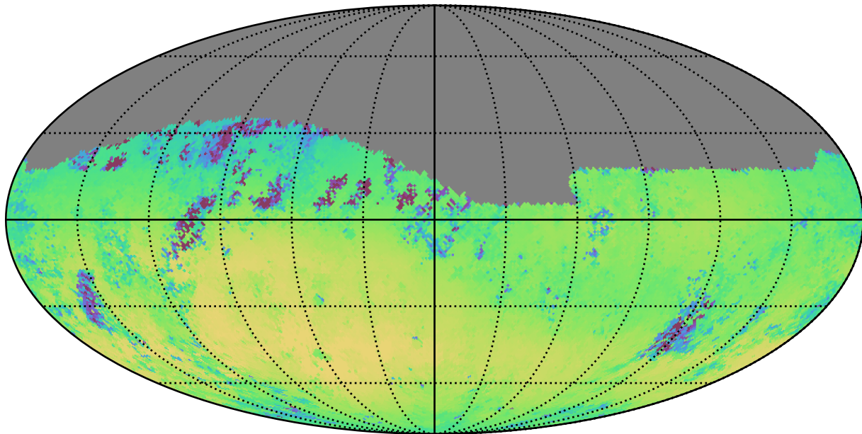
ddf_half_v3.4_10yrs Yr 1 r band: Median skyBrightness
