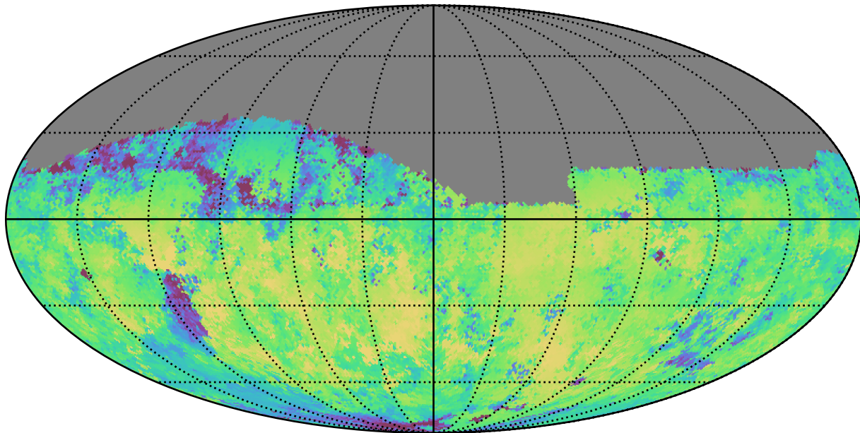
ddf_half_v3.4_10yrs Yr 1 i band: Median skyBrightness
